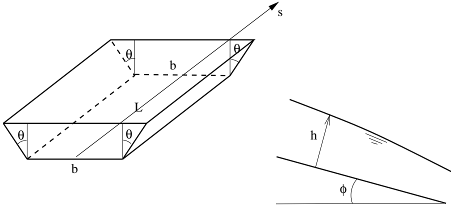
Figure 119: Channel geometry
