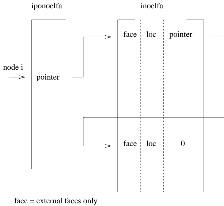
Figure 189: Data structure for all external faces belonging to a given node
