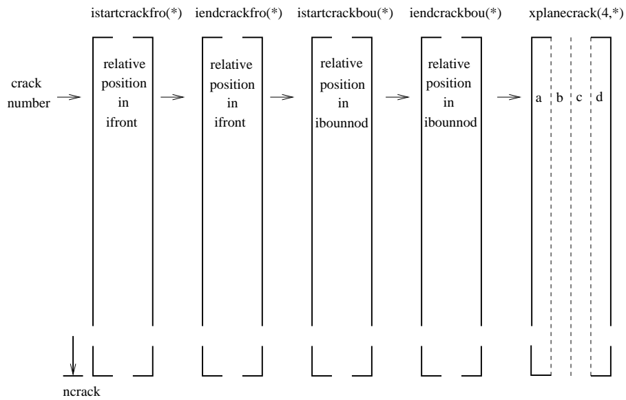
Figure 205: Fields for the crack characteristics
