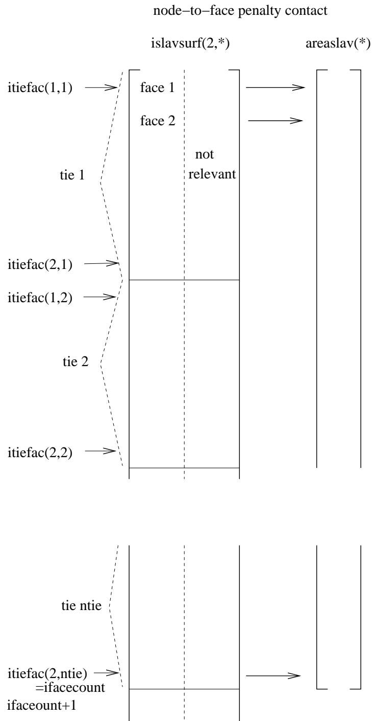
Figure 176: Storage of the slave faces (node-to-face penalty)
