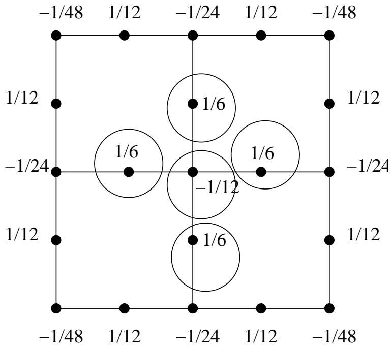
Figure 161: Equivalent forces of a uniform pressure on a plate (4 elements)
