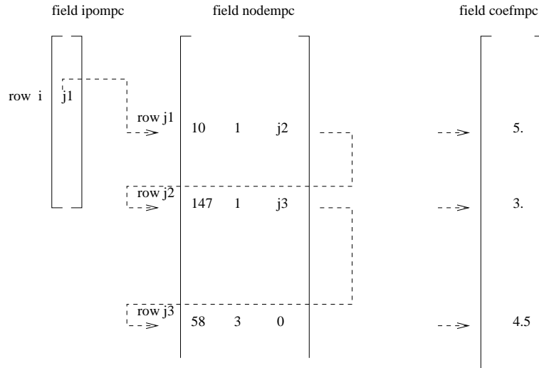
Figure 167: Example of the storage of a linear equation
