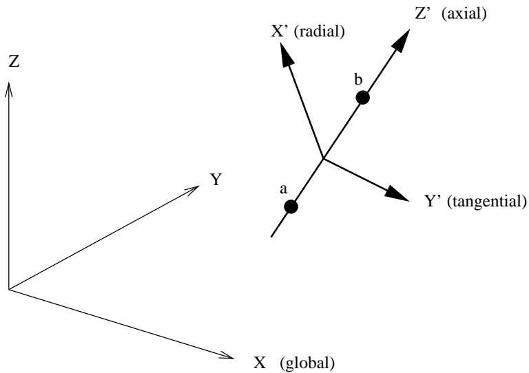
Figure 163: Definition of a cylindrical coordinate system
