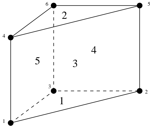
Figure 156: Face numbering for wedge elements
