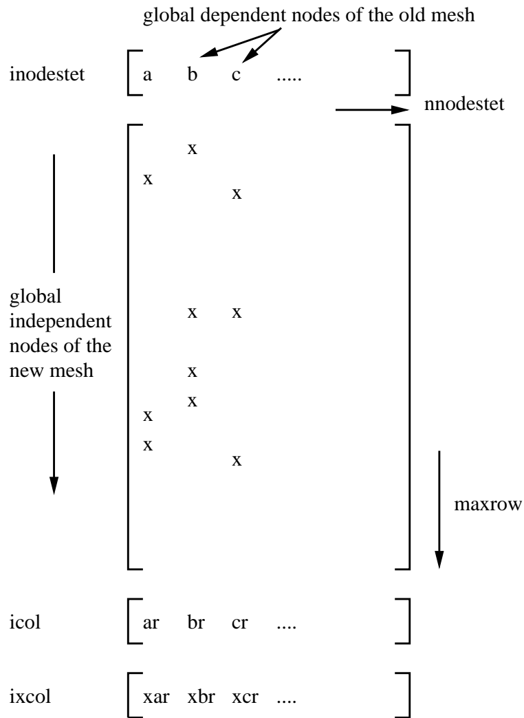
Figure 198: Matrix structure of the connecting equations
