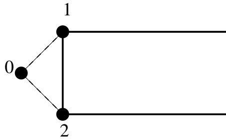
Figure 170: Shell element connection
