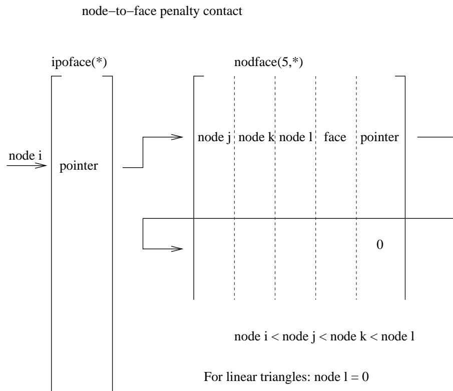
Figure 174: Storage of all faces for the determination of the external faces
