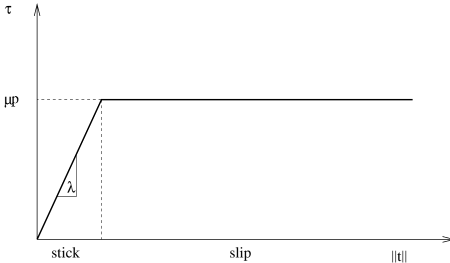
Figure 131: Shear stress versus relative tangential displacement
