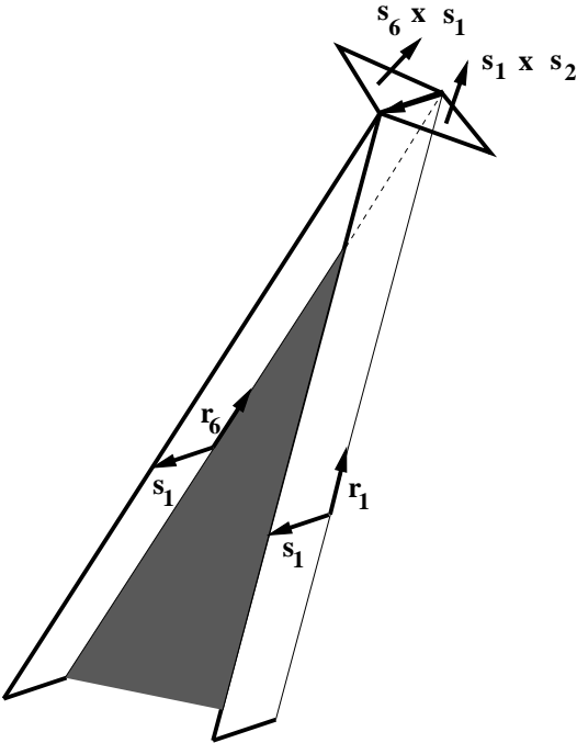
Figure 143: Limits of the return regions for Mohr-Coulomb
