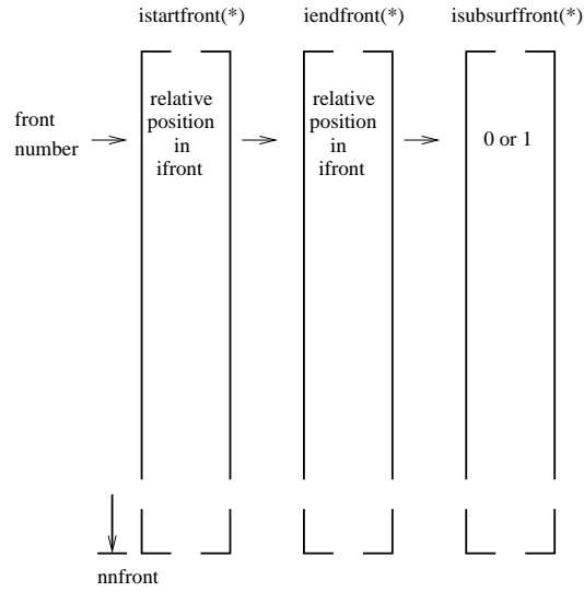
Figure 204: Fields for the front characteristics
