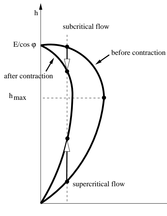
Figure 123: Specific energy at a contraction
