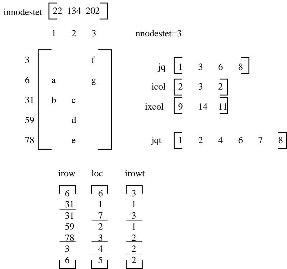
Figure 200: Example for the fields defining the connecting equations
