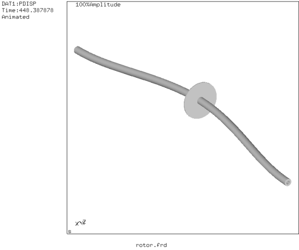
Figure 12: Two-node eigenmode
