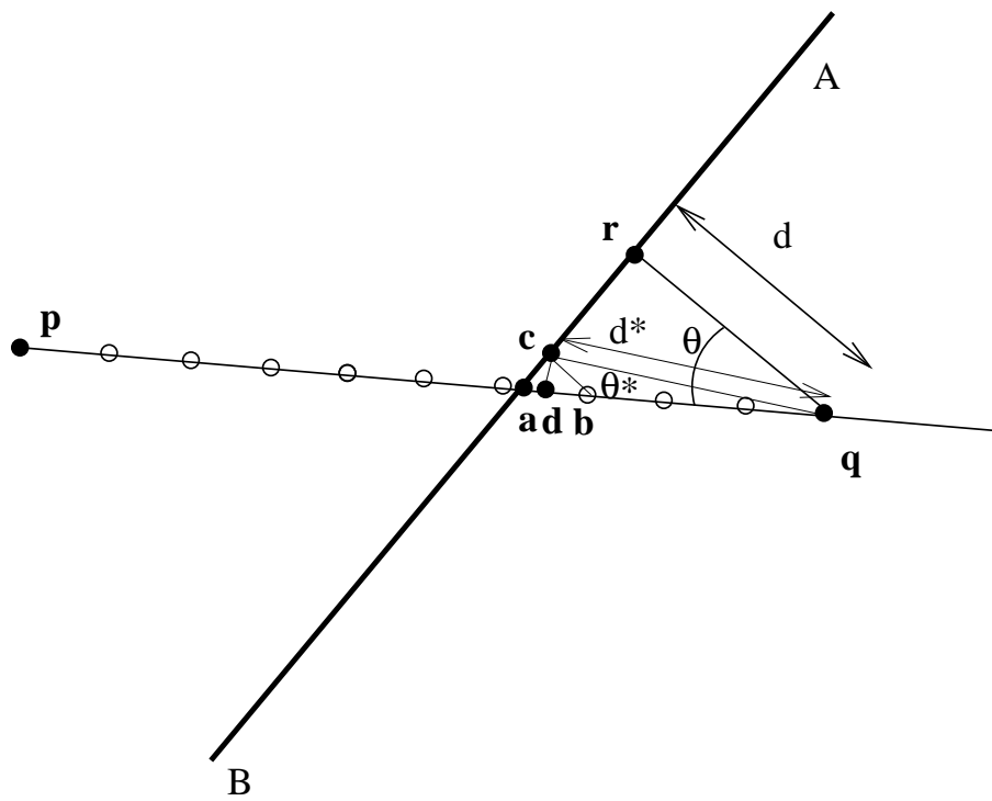
Figure 206: Calculation of a front position external but close to the free surface.
