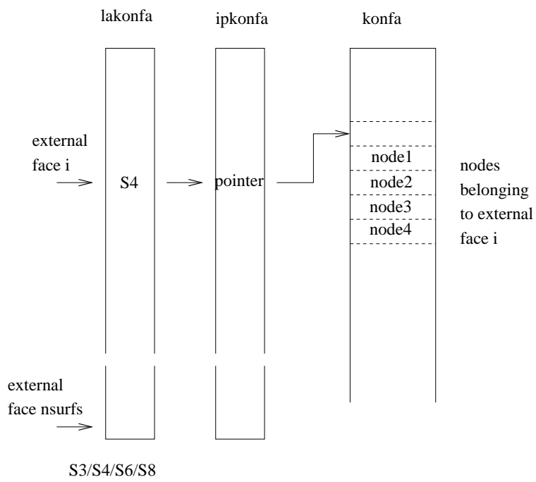
Figure 188: Data structure storing the kind of external face and the nodes belonging to that face
