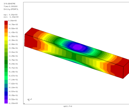
Figure 48: Stress sensitivity after filtering
