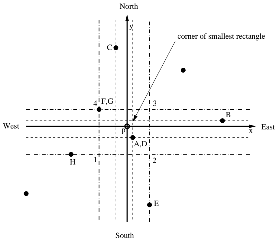
Figure 208: Scheme of the nearest point algorithm
