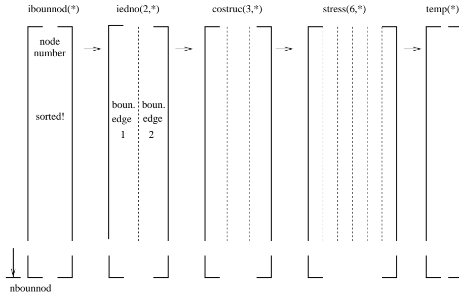
Figure 201: Fields for the boundary nodes and edges
