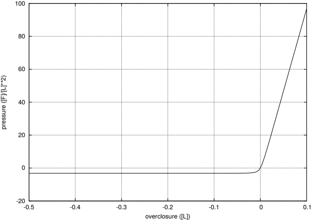
Figure 130: Linear pressure-overclosure relationship
