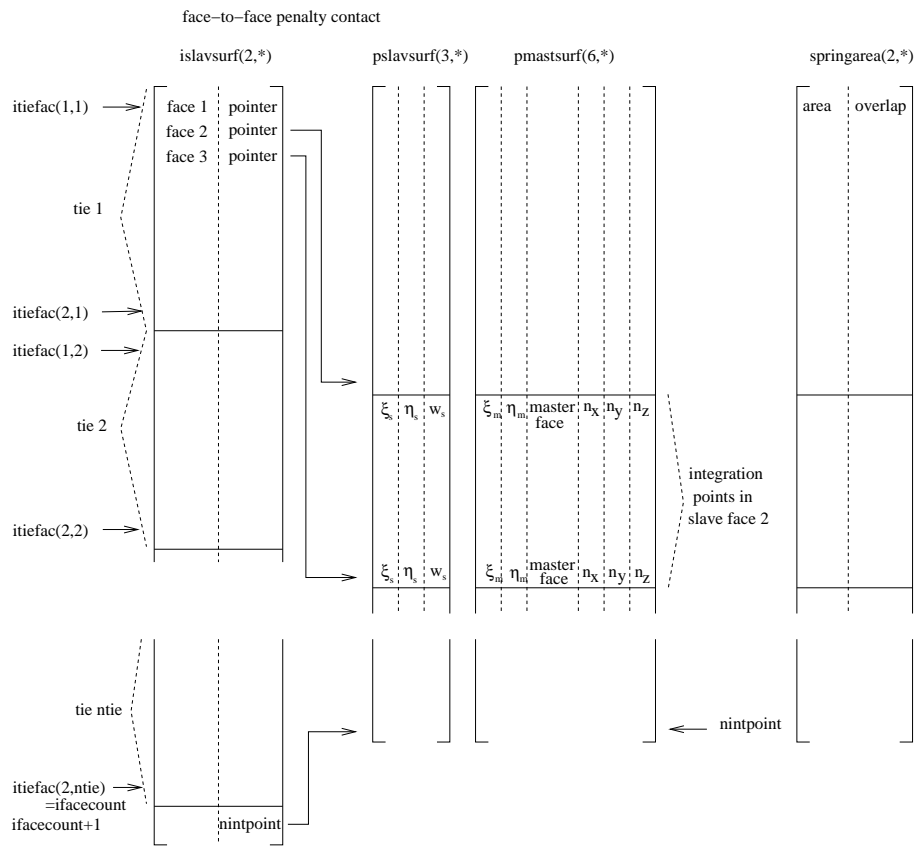
Figure 177: Storage of the slave faces (face-to-face penalty)
