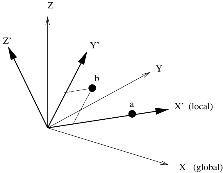
Figure 162: Definition of a rectangular coordinate system
