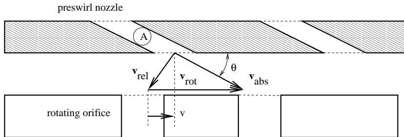
Figure 85: Geometry of the preswirl nozzle fluid section and the orifice it serves
