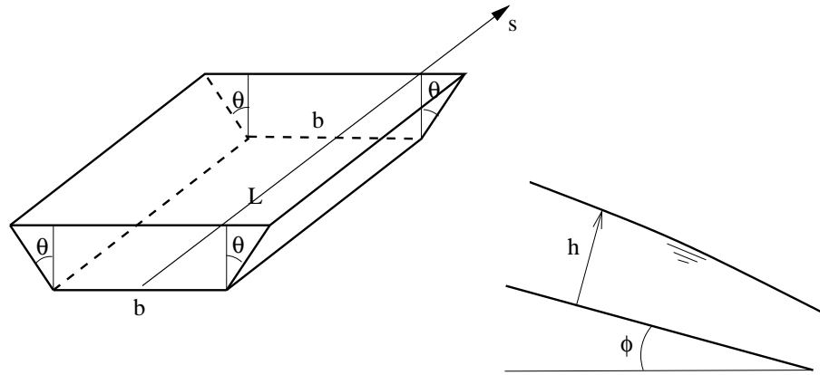
Figure 146: Channel geometry
