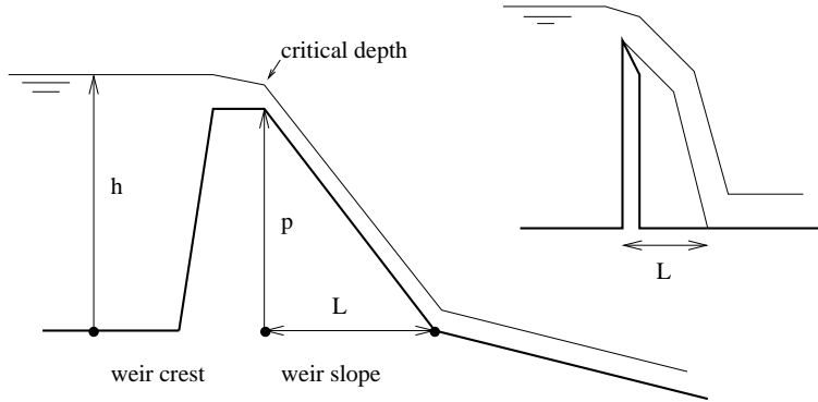
Figure 121: Weir geometry
