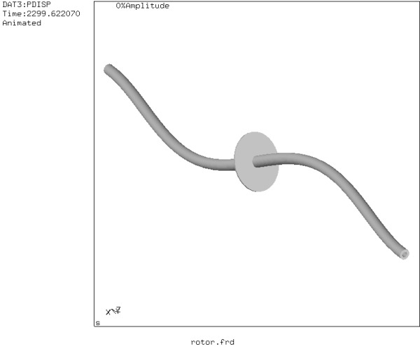
Figure 13: Three-node eigenmode
