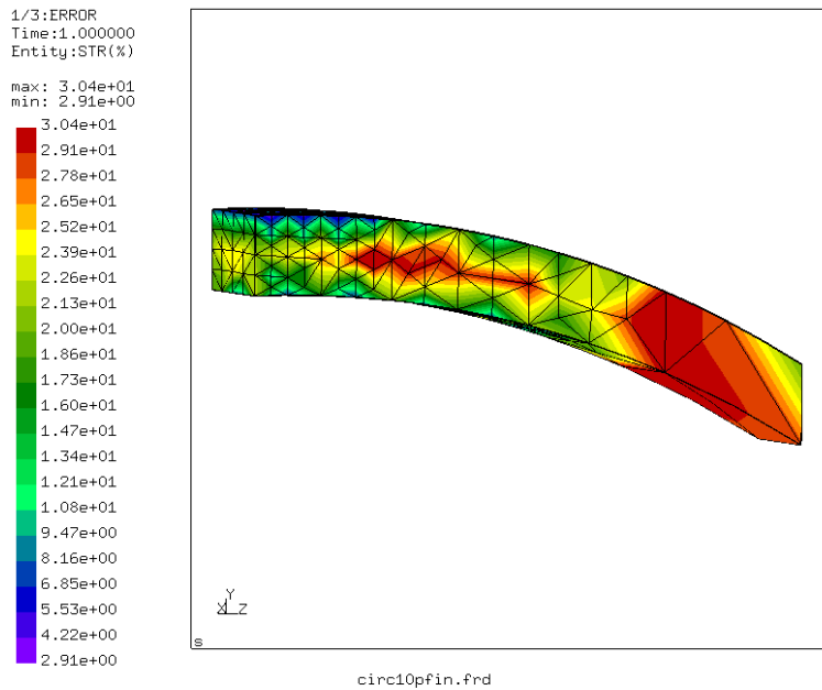
Figure 56: Error estimator for the fine mesh
