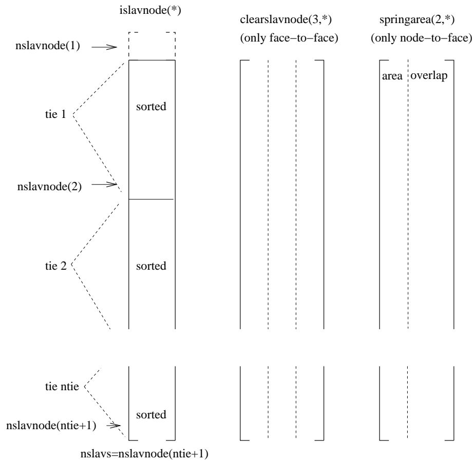
Figure 175: Storage of the slave nodes
