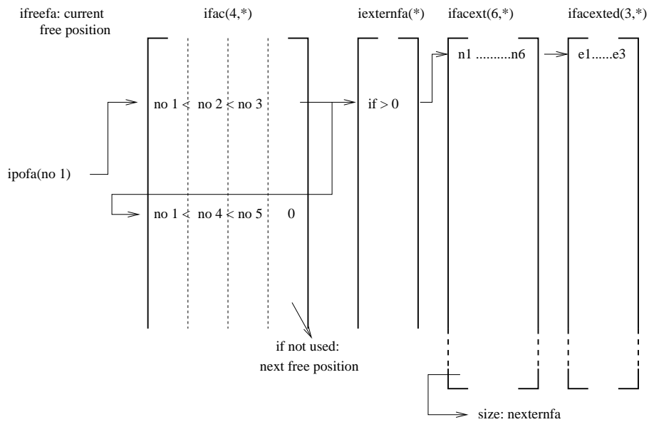
Figure 195: Node per face relationship
