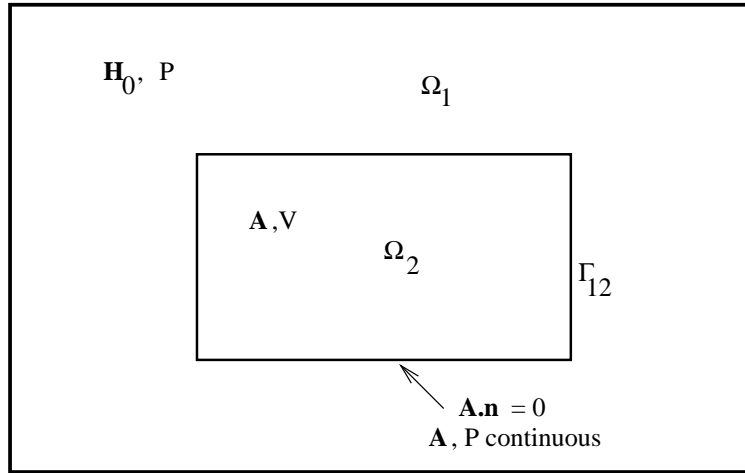
Figure 150: Electromagnetic setup for simply connected bodies
