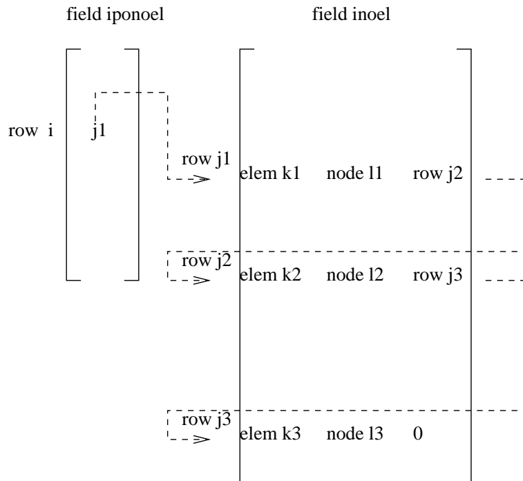
Figure 168: Structures to store all elements to which a given node belongs
