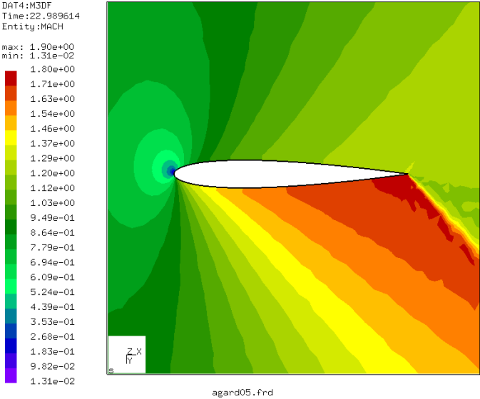
Figure 30: Mach number in the naca012 airfoil flow
