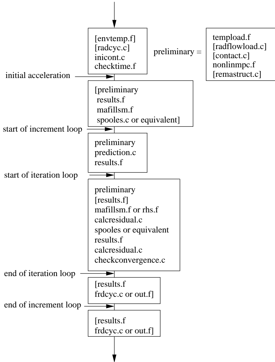
Figure 182: Flow diagram for subroutine nonlinge0
