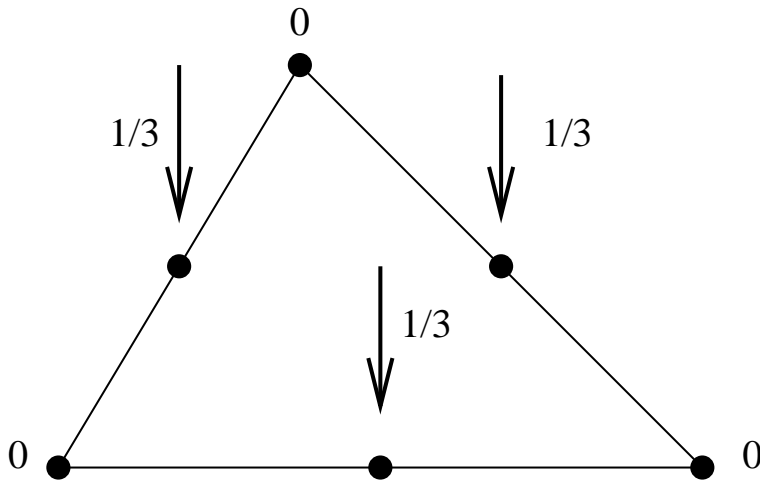
Figure 158: Equivalent nodal forces for a face of a C3D10 element
