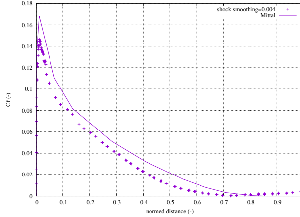
Figure 36: Friction coefficient for laminar viscous flow about a naca012 airfoil
