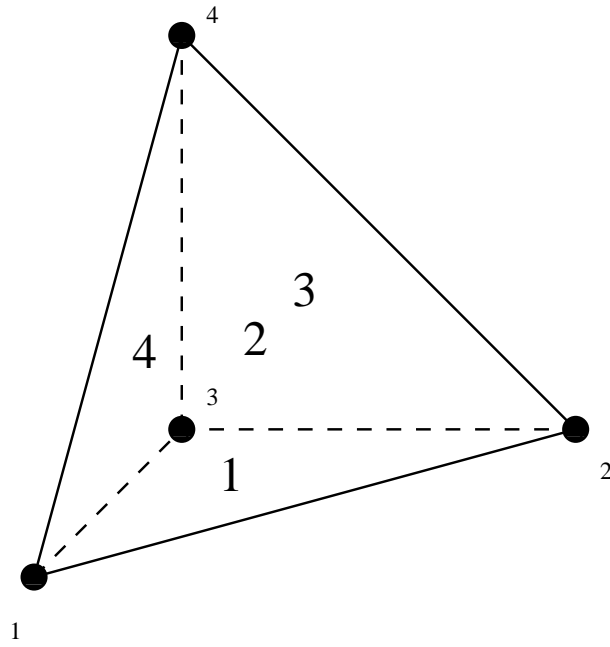
Figure 155: Face numbering for tetrahedral elements
