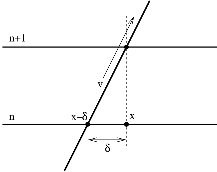
Figure 149: Formulating the equations along characteristics
