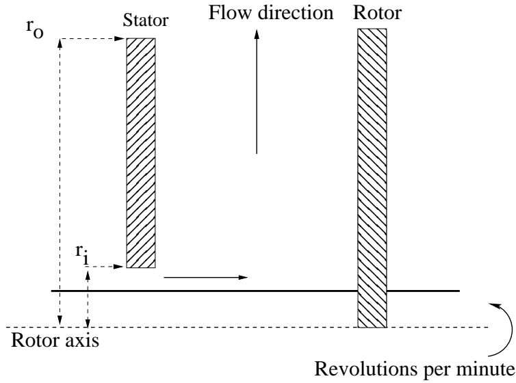
Figure 108: Geometry of a forced vortex
