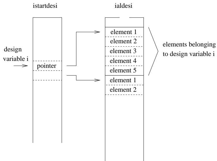
Figure 190: Data structure for all elements belonging to a specific design variable
