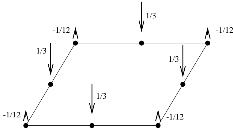
Figure 157: Equivalent nodal forces for a face of a C3D20(R) element
