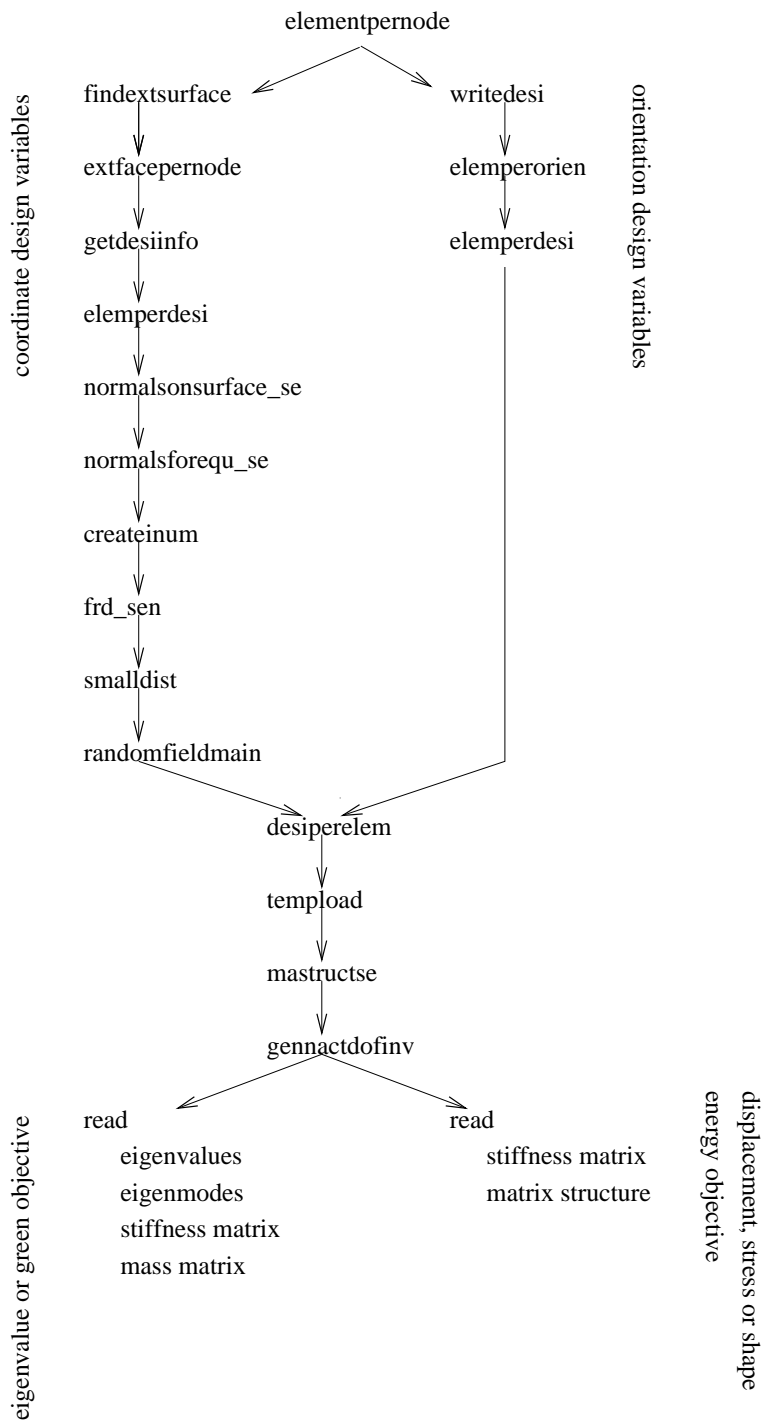
Figure 186: Structure of the preprocessing part
