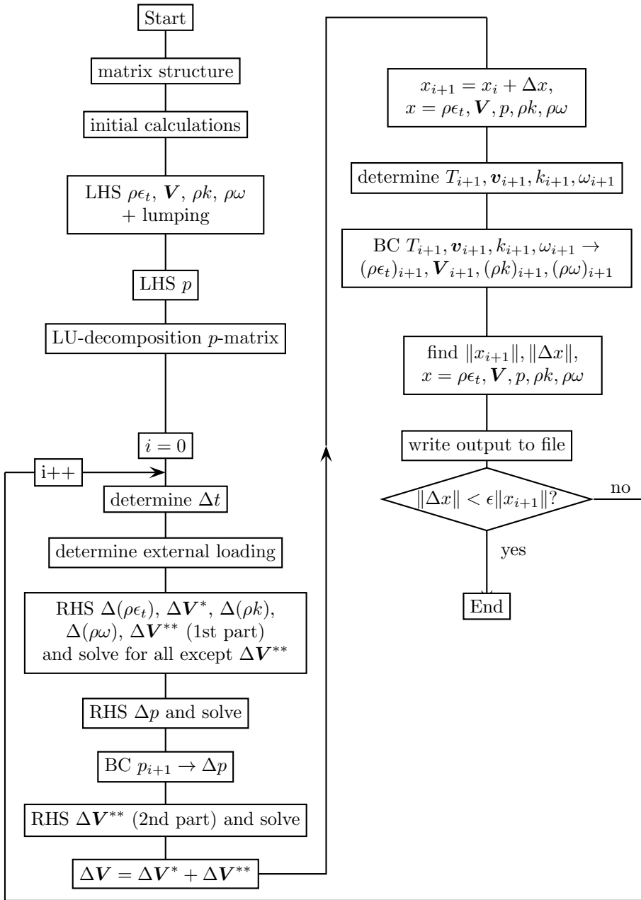
Figure 184: Flow diagram for liquids
