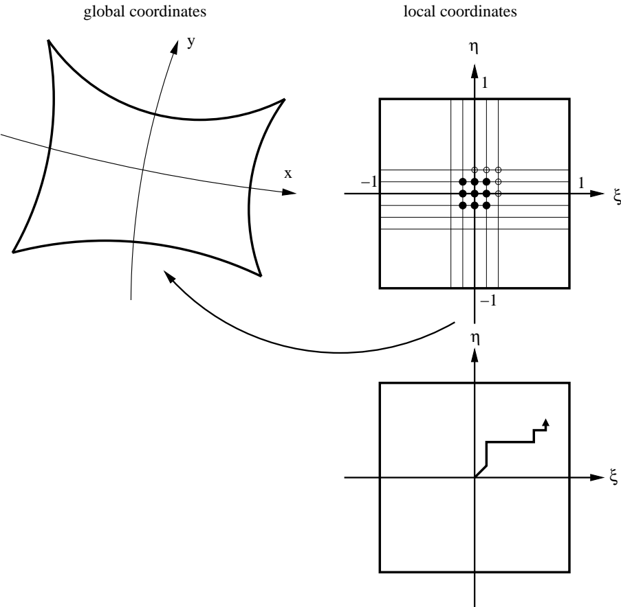
Figure 209: Closest location in an element
