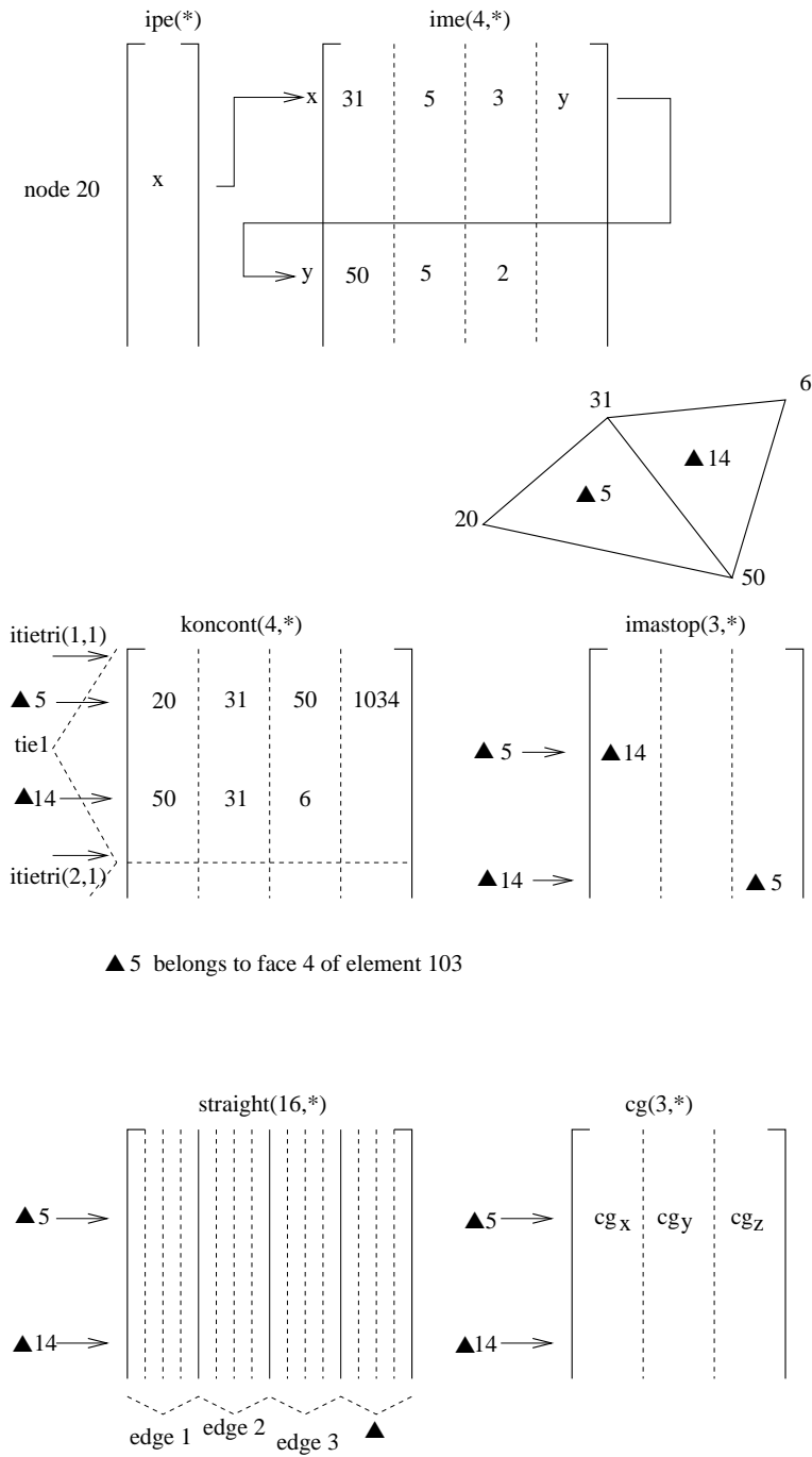
Figure 173: Storage of the triangulation properties
