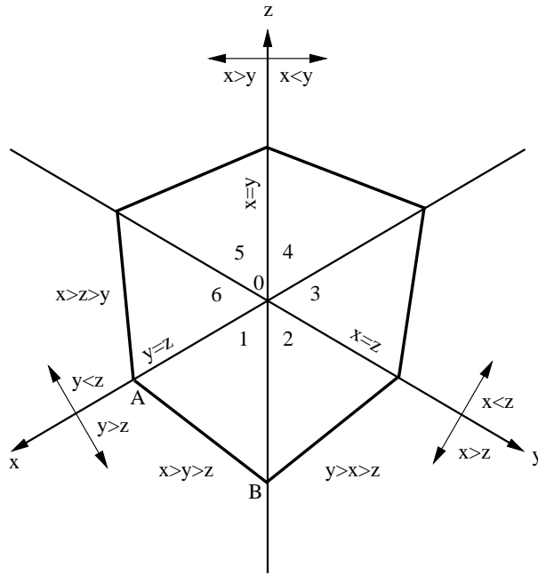
Figure 141: Section plane \perp (1,1,1) through (0,0,0)
