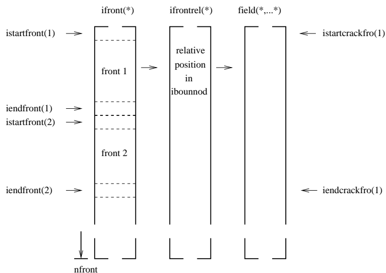
Figure 203: Fields for the front nodes (after analyzing the adjacency relations)
