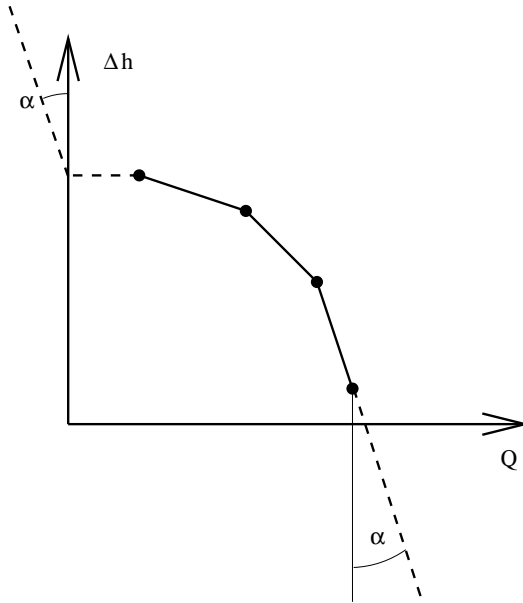
Figure 118: Pump Characteristic
