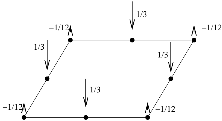
Figure 160: Equivalent forces of a uniform pressure on a plate (1 element)
