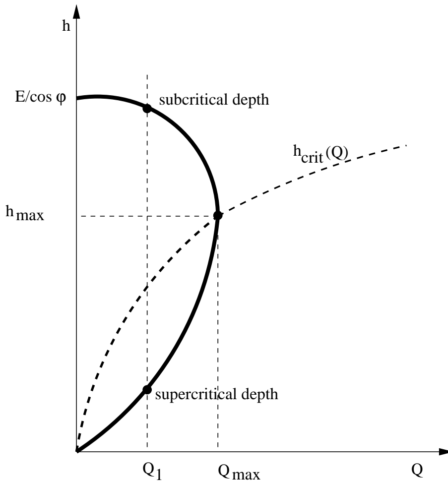
Figure 148: Allowable volumetric flow for a given specific energy
