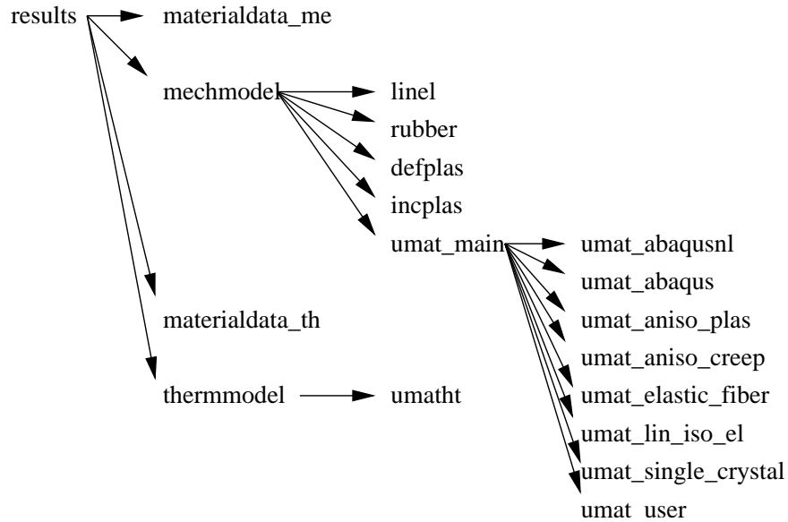
Figure 183: Flow diagram for subroutine results
