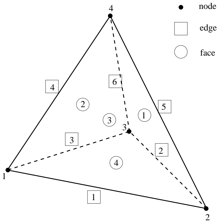
Figure 196: Node, edge and face numbering within a tetrahedral element
