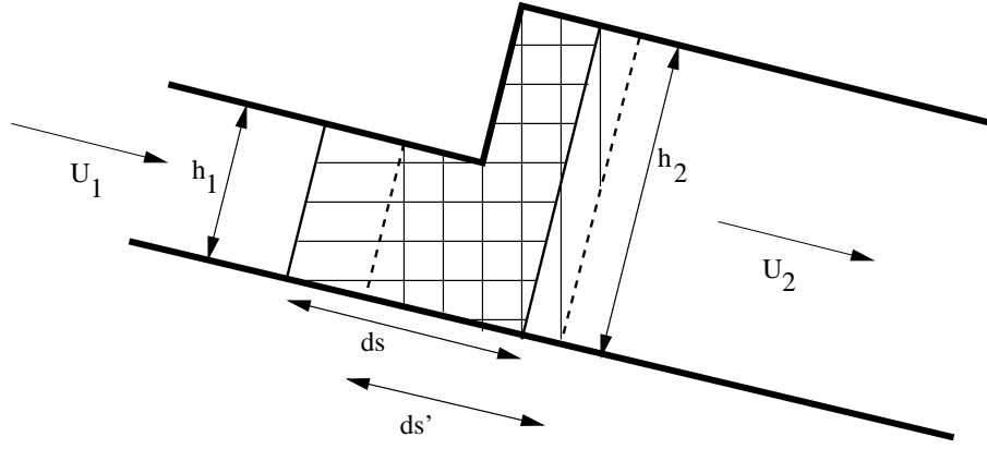
Figure 147: Conservation of momentum at a jump
