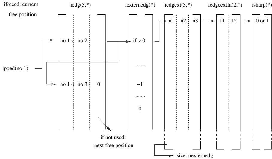
Figure 193: Node per edge relationship
