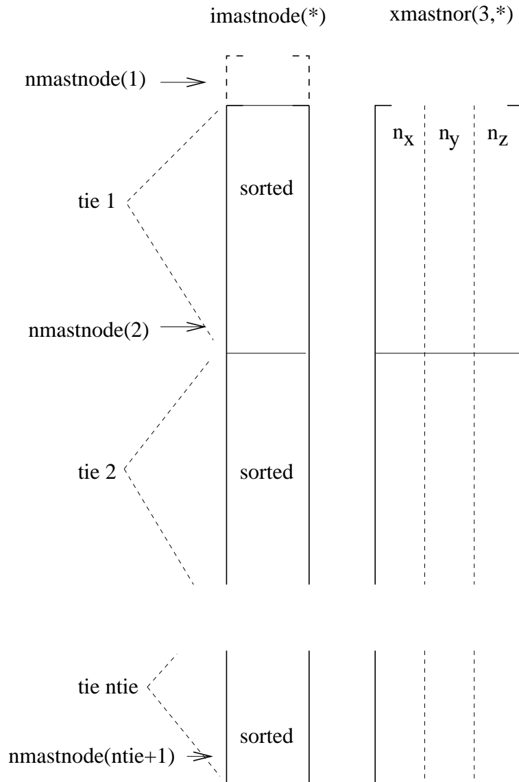
Figure 179: Storage of the master nodes
