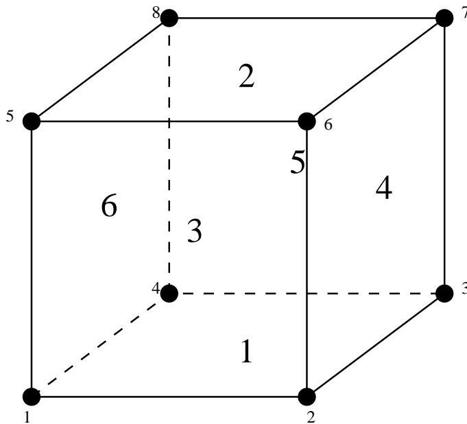
Figure 154: Face numbering for hexahedral elements
