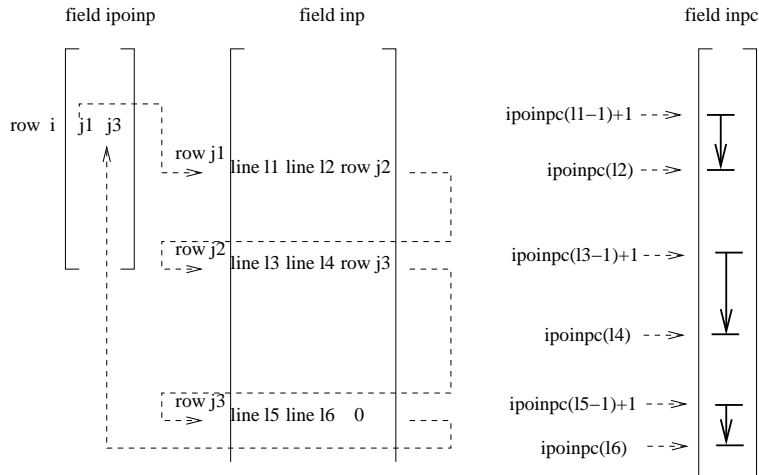
Figure 166: Reading the lines for keyword entry i
