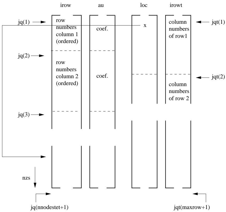
Figure 199: Fields describing the matrix structure
