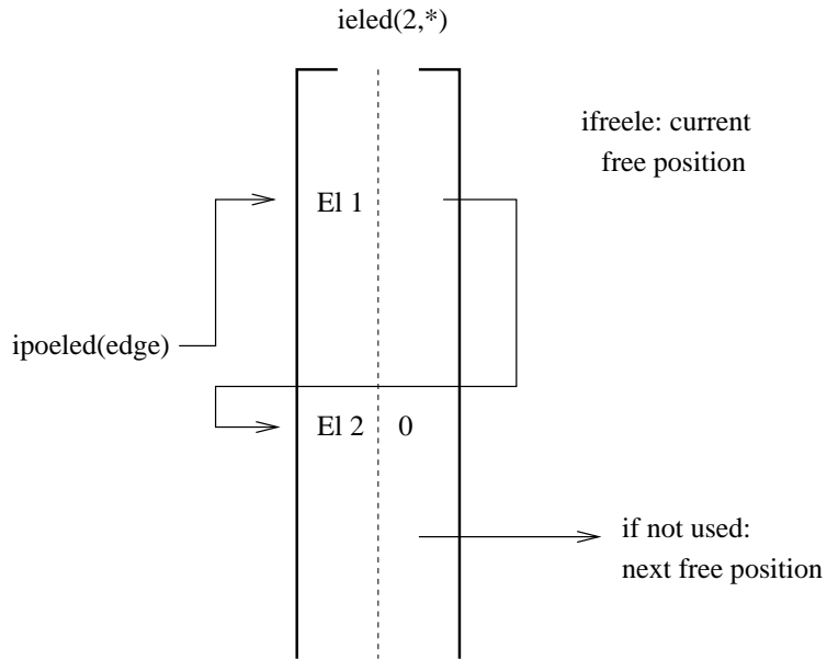
Figure 194: Element per edge relationship
