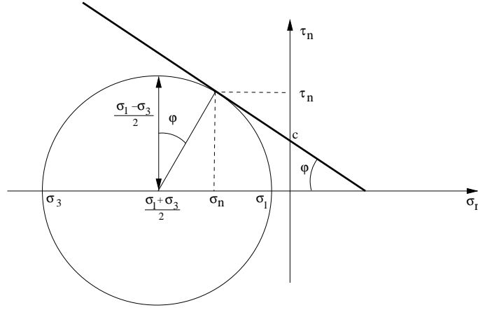
Figure 140: Mohr-Coulomb yield surface
