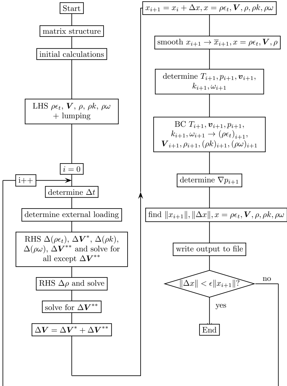
Figure 185: Flow diagram for compressible fluids
