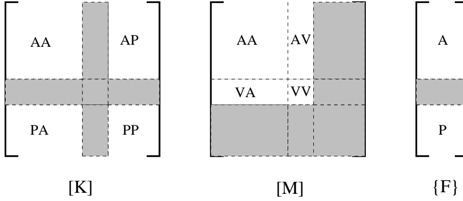
Figure 152: Nonzero parts of the governing matrices
