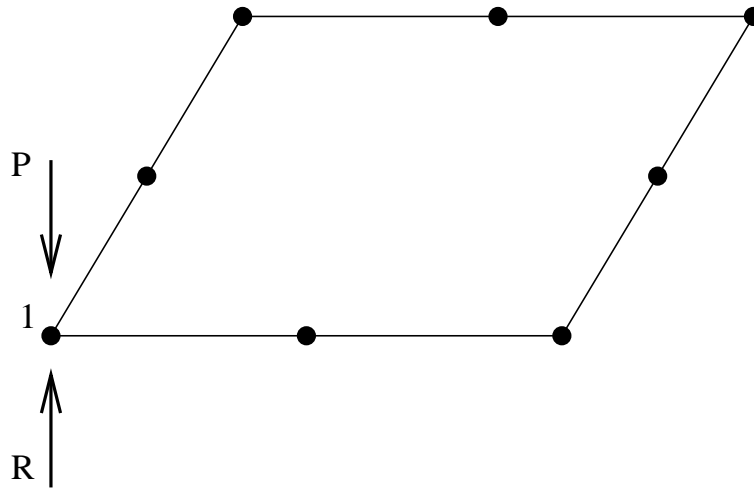
Figure 159: Point load in a node belonging to a 8-noded face
