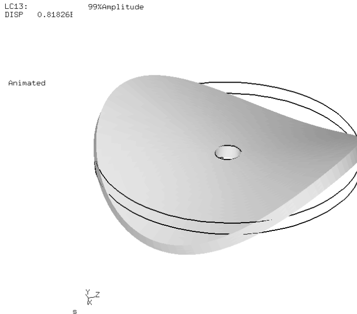
Figure 145: Eigenmode for a full disk with a nodal diameter of two
