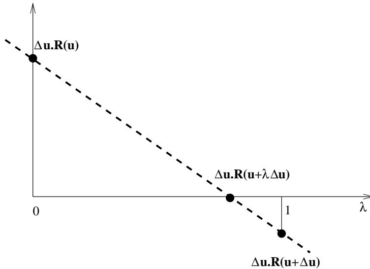
Figure 153: Principle of the line search method
