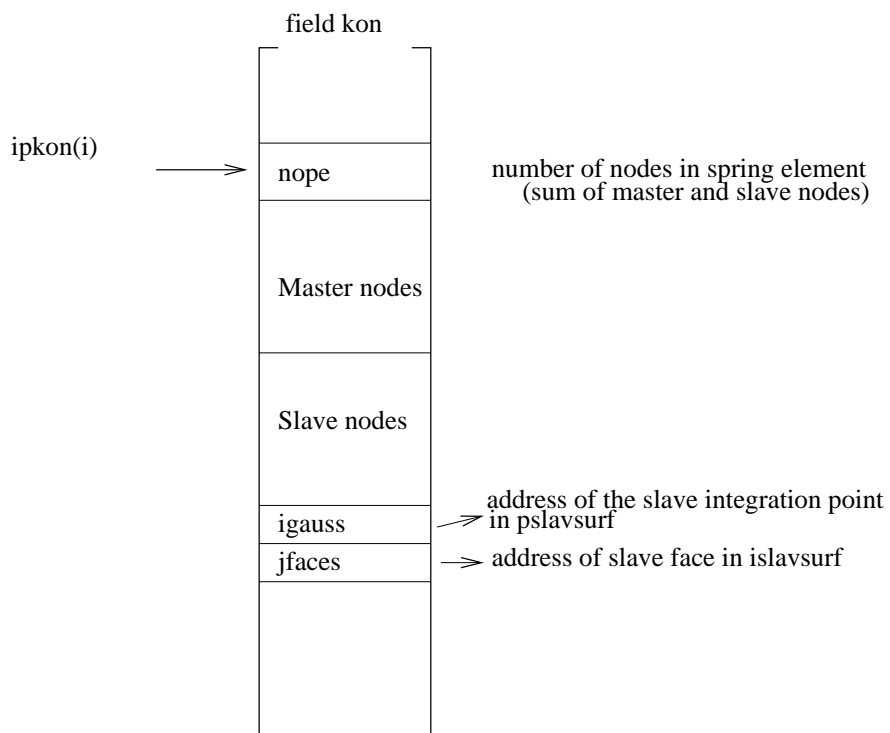
Figure 181: Topology of the face-to-face penalty contact elements
