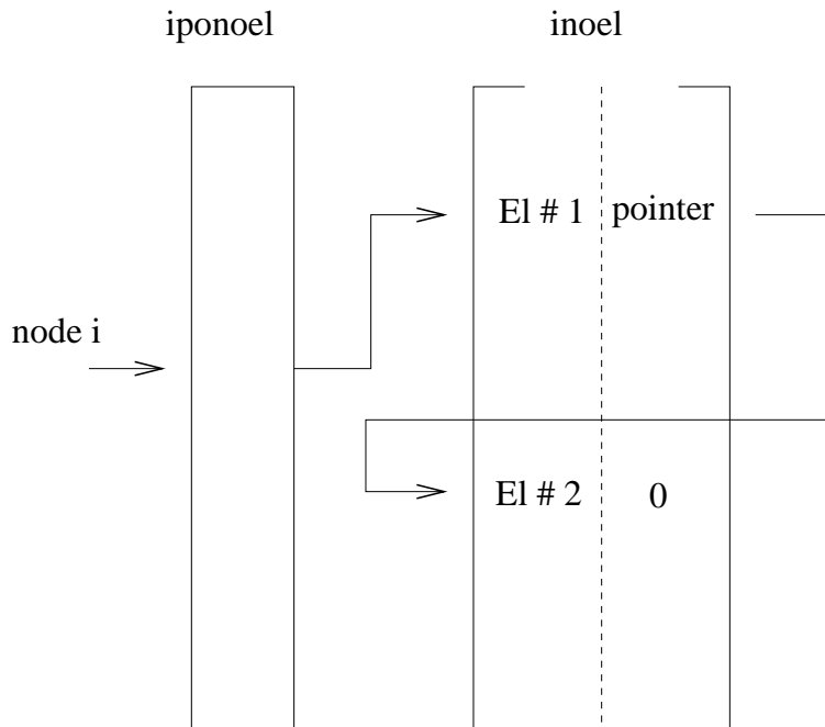
Figure 187: Data structure for all elements belonging to a given node
